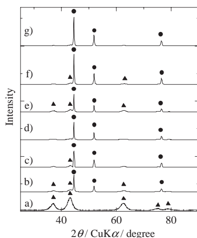
Figure 1. XRD patterns of the obtained particles by a) FT-SCW method and reduction of NiO b) for 5 min, c) for 30 min, d) for 60 min with 0.69 g of HCOOH, e) with 0.37 g of HCOOH, f) with 1.38 g of HCOOH, and g) with 2.76 g of HCOOH for 30 min. Circle and triangle denote Ni and NiO, respectively.
