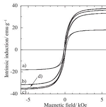
Figure 3. Typical VSM results of the obtained particles by reduction of NiO a) for 5 min, b) for 30 min, c) for 60 min with 0.69 g of HCOOH, and d) with 2.76 g of HCOOH for 30 min.
