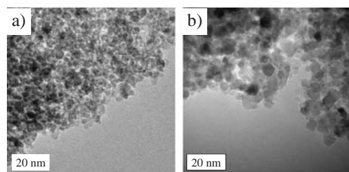
Figure 2. Typical TEM images of the obtained particles by a) FT-SCW method and b) reduction of NiO for 60 min with 0.69 g of HCOOH.
